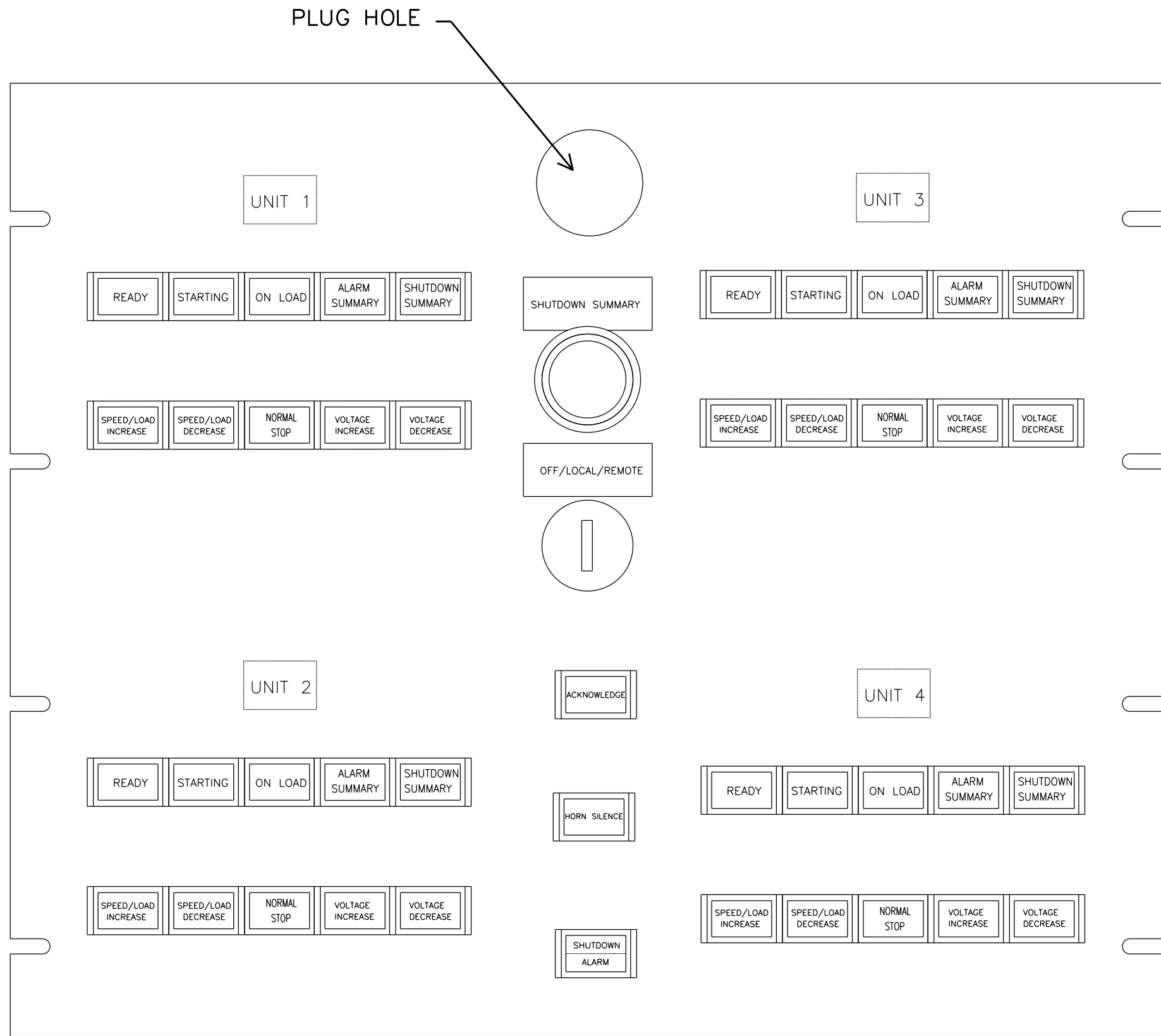
FRONT VIEW
